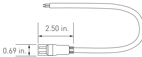
Hard-Wire Universal Power Feed Splice Connector* AL-11-99-9902-SC-24IN (24 in. - White) AL-11-99-9902-SC-96IN (96 in. - White)
