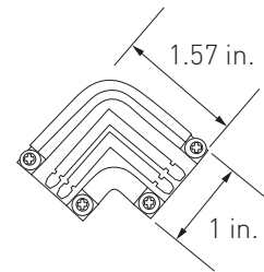
Universal L-Connector with Screws - 90 Degree AL-11-99-9902-LC
