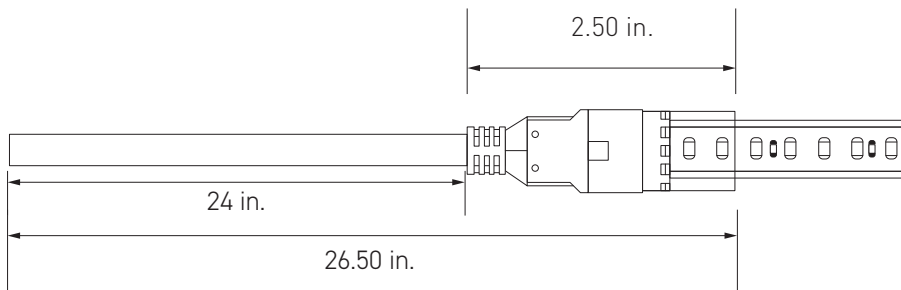
Hard-Wire Configuration (UL 1598)
