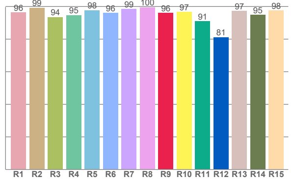
CRI: 97.0 (R1-R8)
