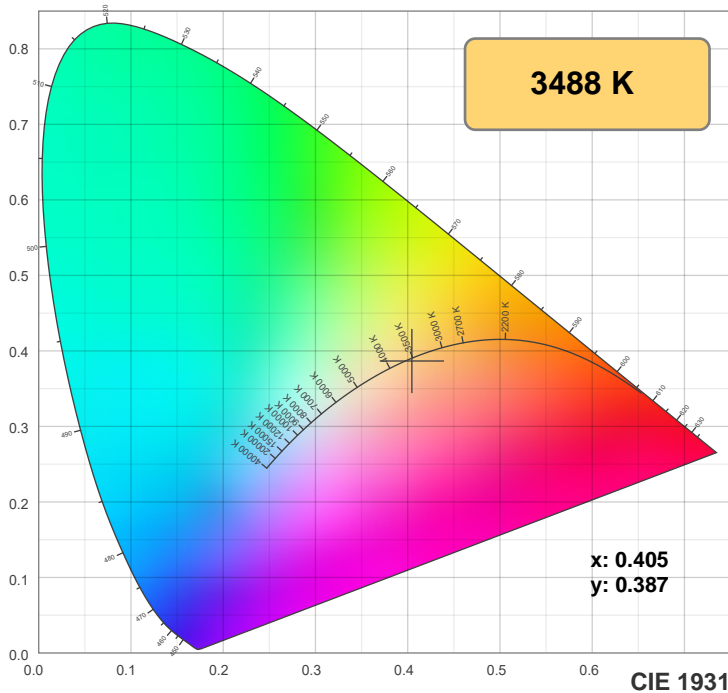
TM-30: 93.4
