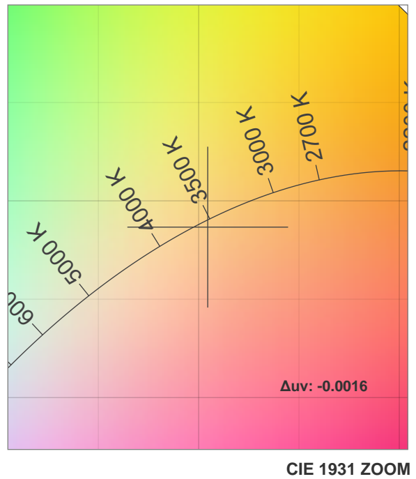
CRI: 97.0 (R1-R8)
